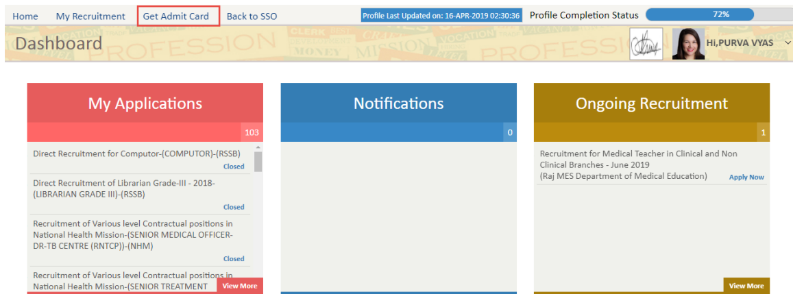
Fig 3 : Candidate Dashboard
