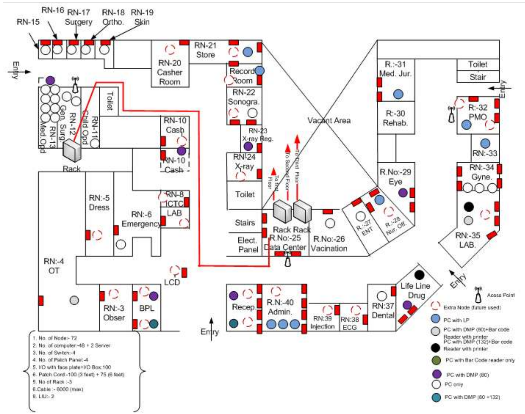
DH7.1: Network Layout of Ground Floor, Kanwatia Hospital, Jaipur
