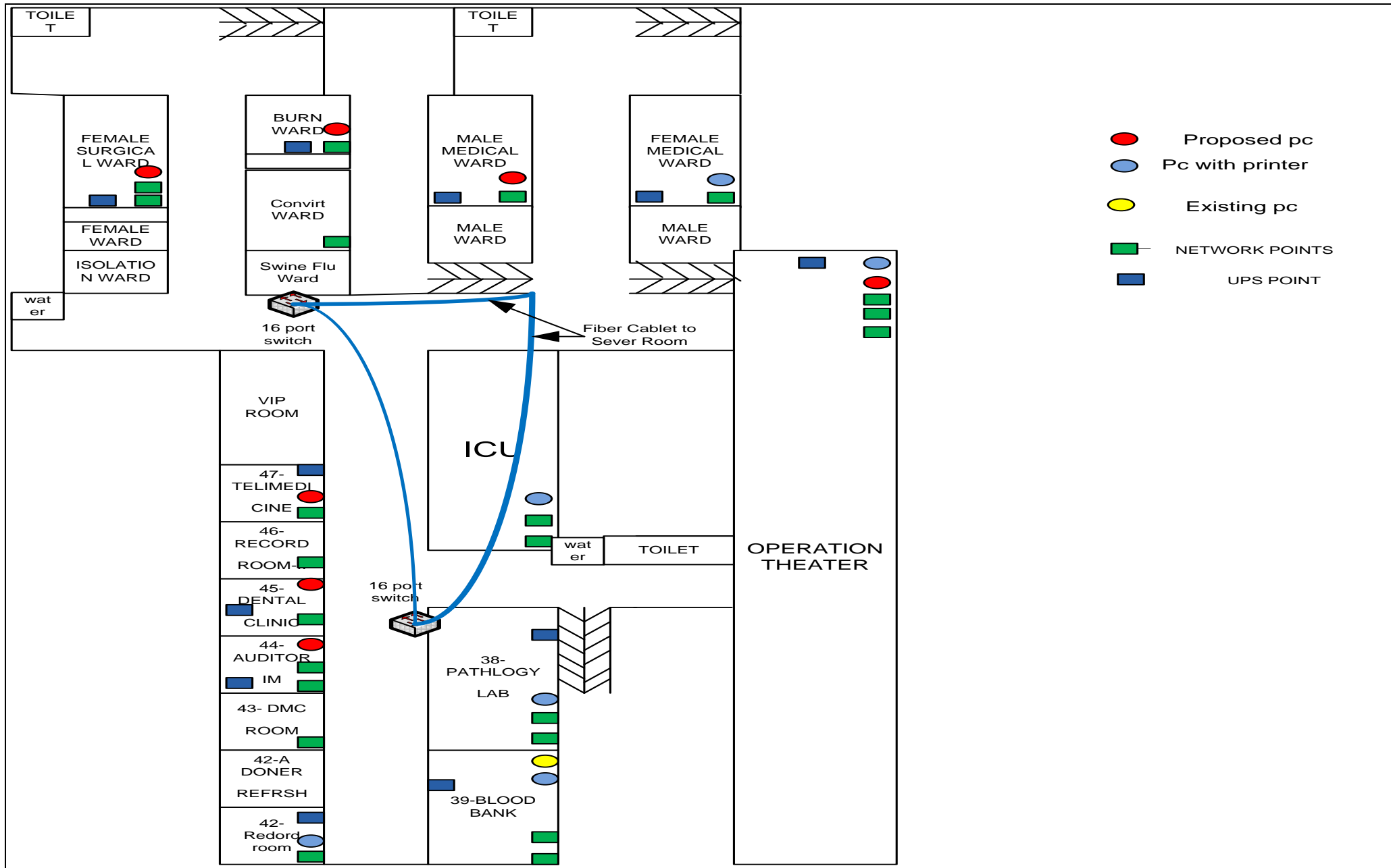
DH9.2: Layout and facilities of First Floor, Sri Ganganagar Hospital
