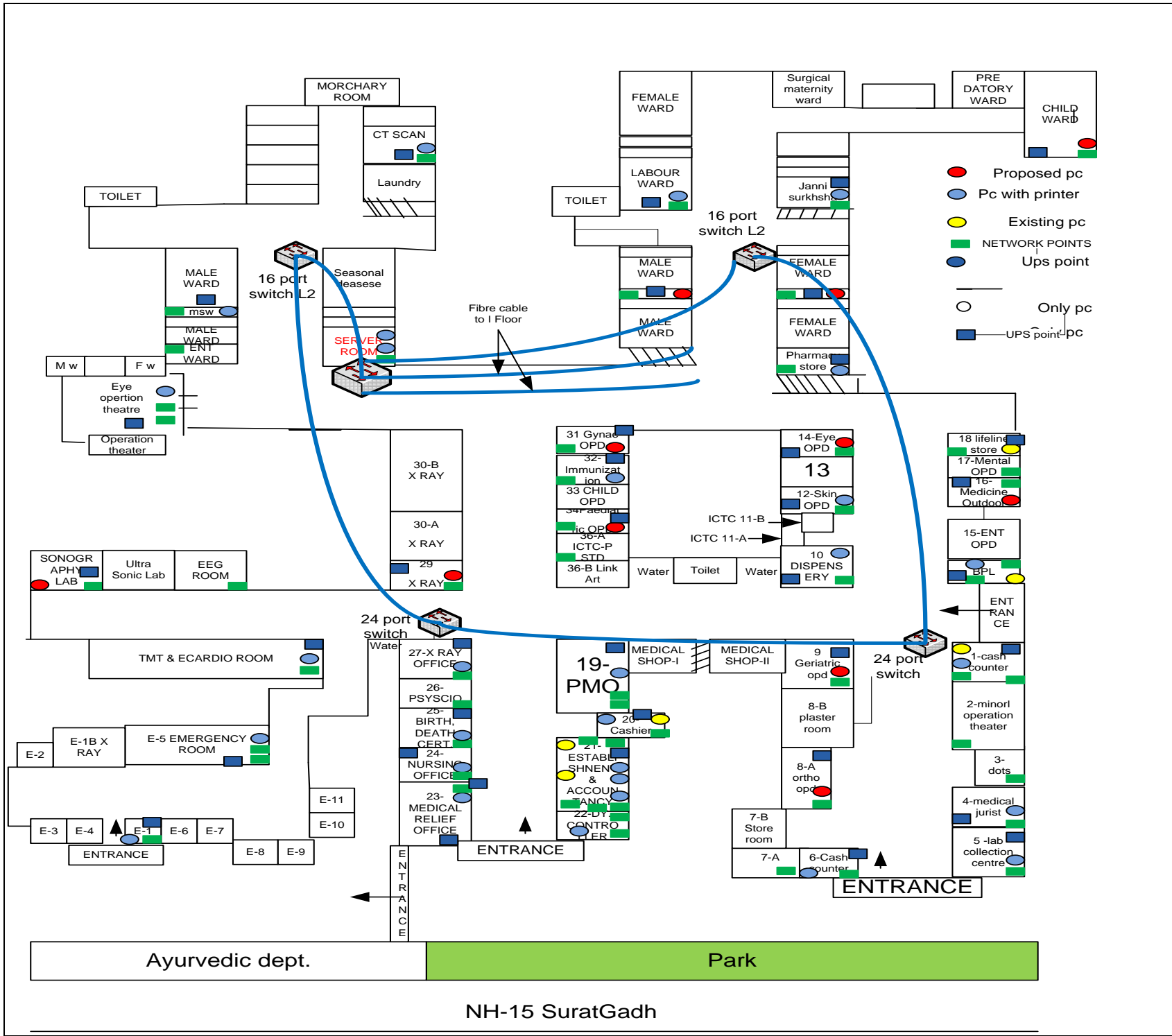
DH9.1: Network Layout of Ground Floor, Sri Ganganagar Hospital
