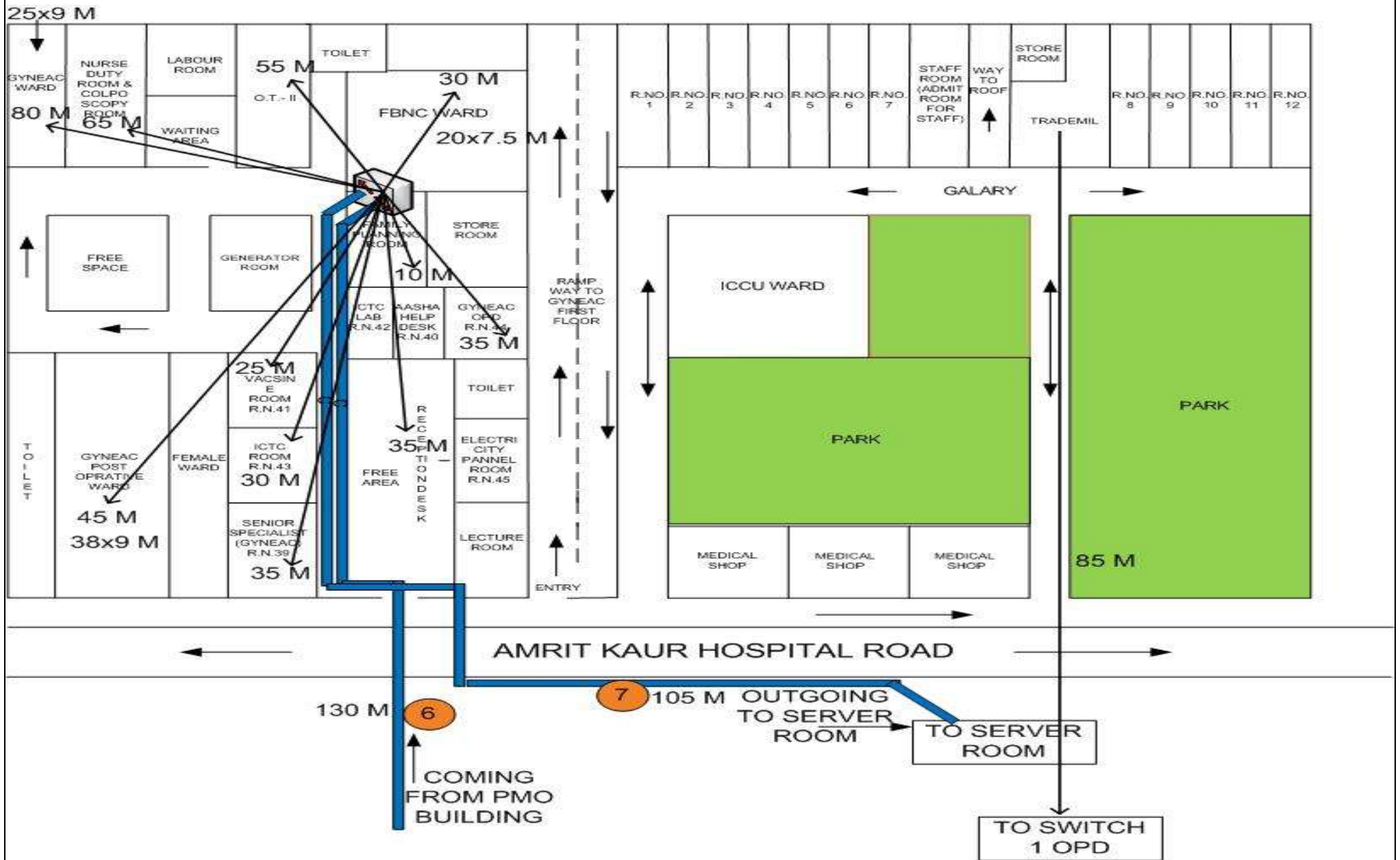
DH8.2: Network Layout of Ground Floor of Gynae & Cottage cum ICU Building, Ajmer Hospital
