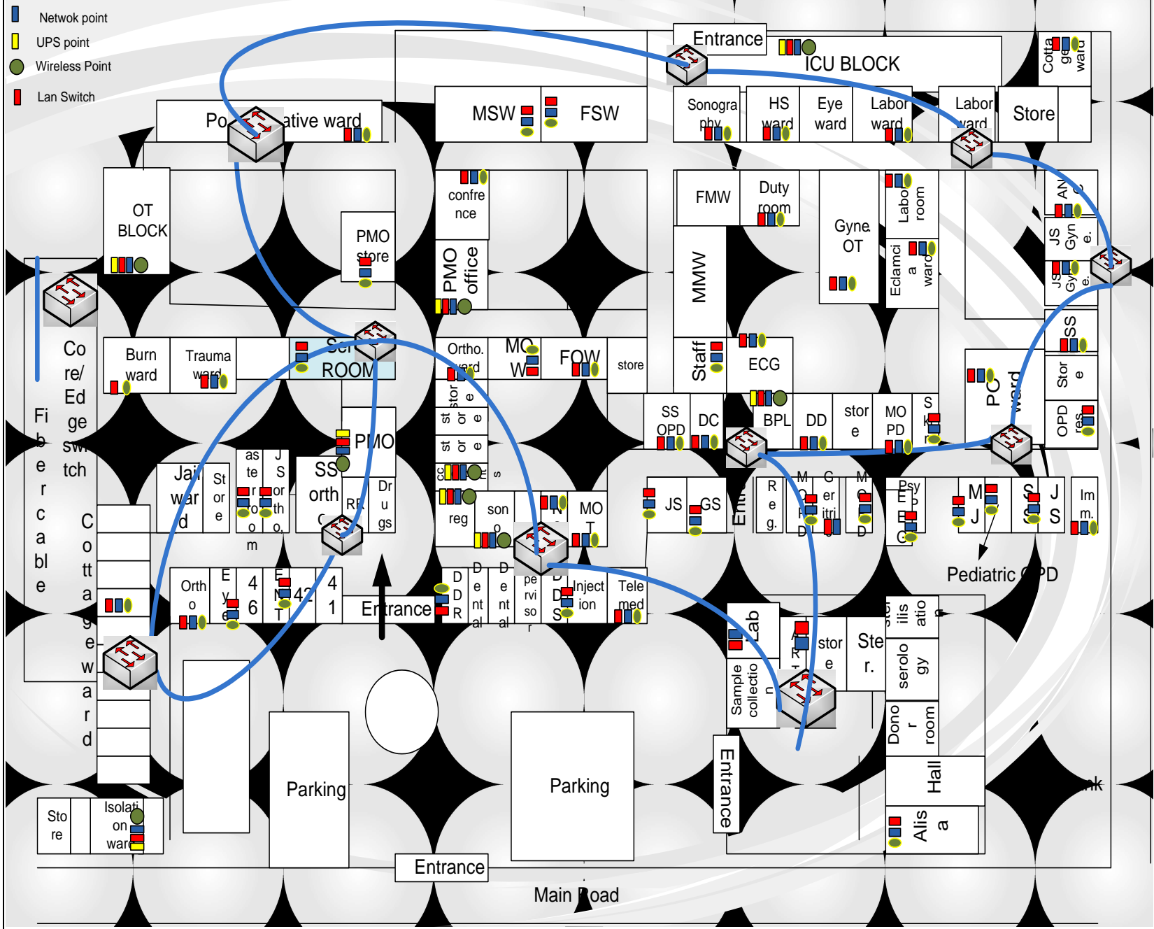
DH5.1: Proposed Network layout of ground floor, Pali Hospital
