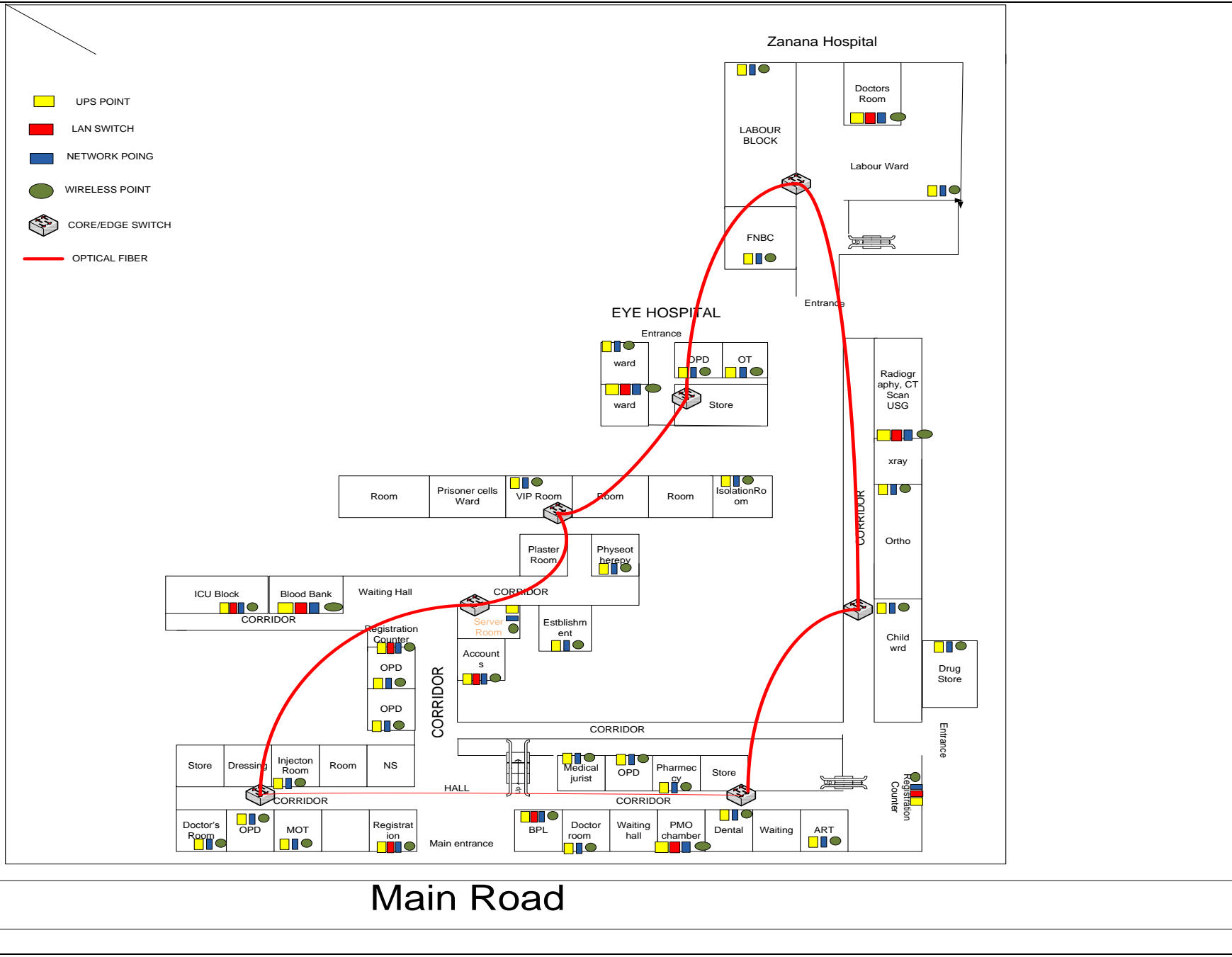
DH3.1: Proposed Network layout of ground Floor, Banswara Hospital
