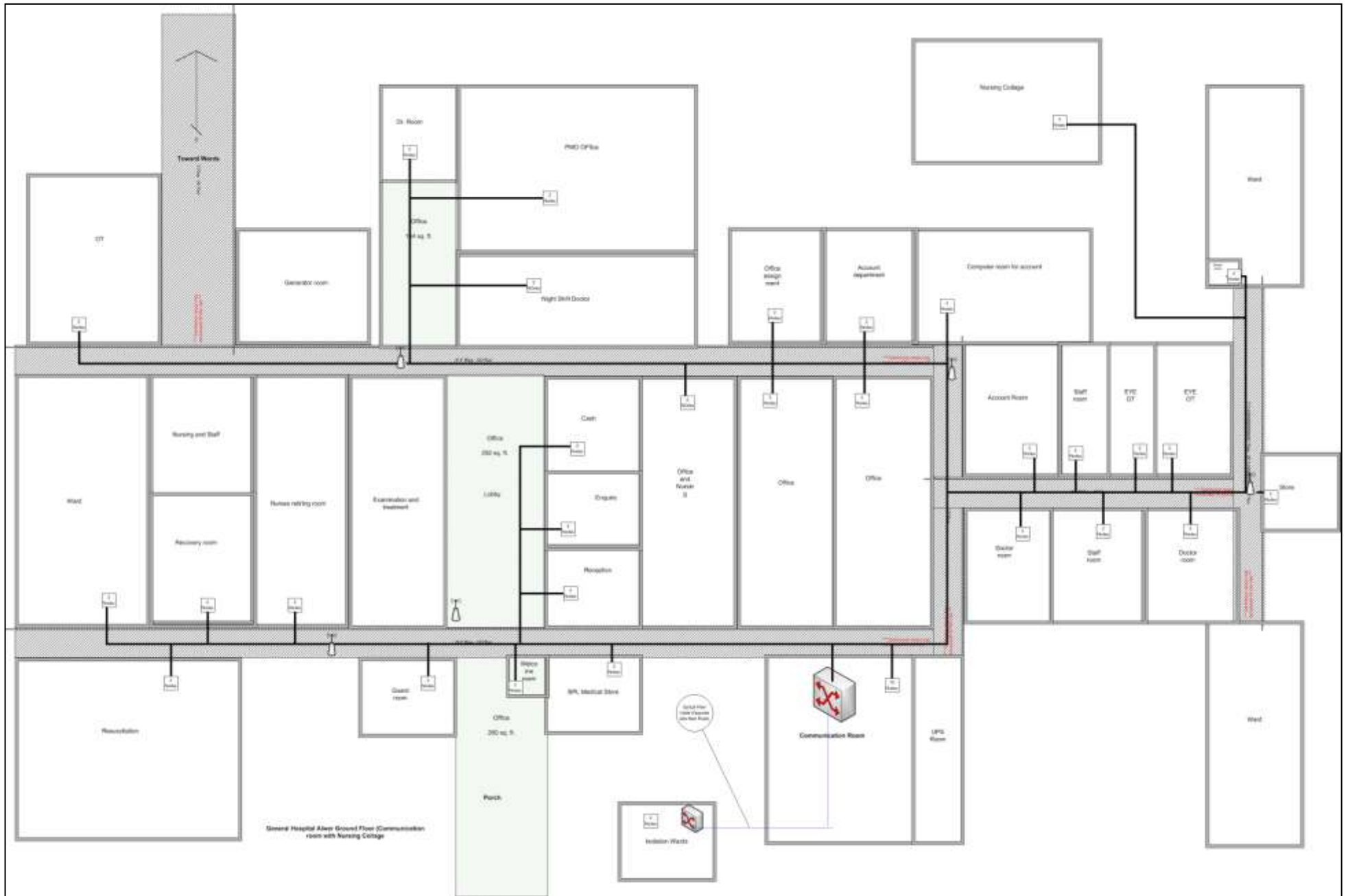
DH1.1: Networking layout of ground floor (Emergency Side), Alwar General Hospital
